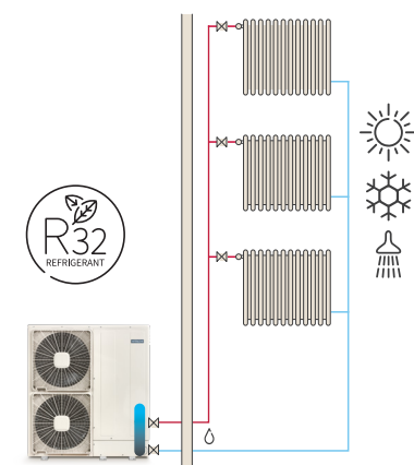
Outdoor unit R32 Heat exchanger R32/ H20
